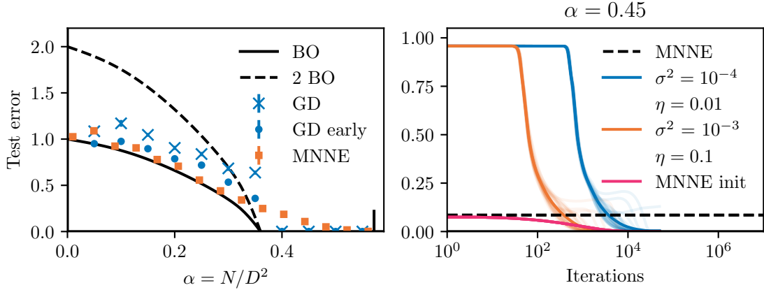
FIG. 6. (Left) Comparison between the test error achieved by GD initialised with small norm (blue crosses, d = L = 50 , maximum iterations T = 10^4 , learning rate \eta = 0.2 , initialisation norm \sigma^2 = 10^{-4} ) and its early stopped version (blue dots) averaged over 16 instances, the test error of the MNNE (orange squares, d = L = 50 ) and of the BO test error (solid black line, dashed lines is twice the BO error corresponding to the error of the Gibbs sampler) for \beta = 1 , \rho = 0.2 and \Delta = 0 . We observe that the MNNE performs slightly better than GD with small initialisation up to roughly the BO strong recovery thresholds, while for larger \alpha GD becomes better, and notably has a better strong recovery threshold than MNNE. (Right) Comparison between the MNNE and several runs of GD with small initialisation (maximum iterations \tau = 20000 ), all on the same instance of the data and ground-truth with d = L = 50 , \rho = 0.2 and \Delta = 0 . We perform this comparison at \alpha = 0.45 , where the left panel suggests that GD will achieve zero error, while MNNE does not. We run GD from 2 different initialisation magnitudes \sigma^2 = 10^{-3}, 10^{-4} (orange and blue curves, thick curves mark the average), and we also run GD from the MNNE initialisation (see main text for a precise definition). We observe that in all cases GD outperforms MNNE at convergence. The Bayes-optimal curves are plotted using Result 2 and (24). The performance of MNNE and GD are given by (13) applied to the output of the respective algorithm.
