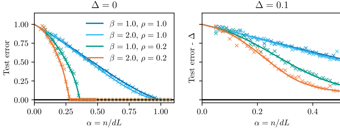
FIG. 3. Comparison between the BO test error and the test error of GAMP-RIE (Algorithm 1) for two choices of the aspect ratio \beta = \max(d, L)/\min(d, L) = 1, 2 and the width ratio \rho = r/\min(d, L) = 0.2, 1 both in the noiseless \Delta = 0 (left) and noisy \Delta = 0.1 (right) case. Solid lines are the theoretical prediction from (24). The crosses represent numerical experiments for the test error measured after iterating GAMP-RIE until convergence, on instances of size \min(d, L) = 100 , with initialisation from the prior distribution. Each point is a run over a single realisation of the data and ground truth. The Bayes-optimal curves are plotted using Result 2 and (24). The performance of GAMP-RIE is given by (14) applied to the output of Algorithm 1.
