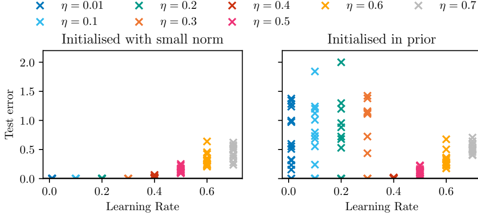
FIG. 11. Test error as a function of the learning rate for GD initialised with small norm ( left ) or in the prior ( right ). Here D = 50 , \beta = 1 , \rho = 0.2 , \alpha = 0.44 . In this regime we expect GAMP-RIE to achieve zero error. We can see how choosing the right learning rate influences the performance of the model rather drastically.
