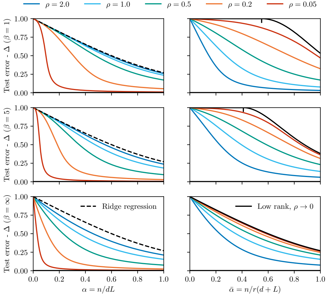
FIG. 9. Same as Figure 1, only with \Delta = 0.1 .
