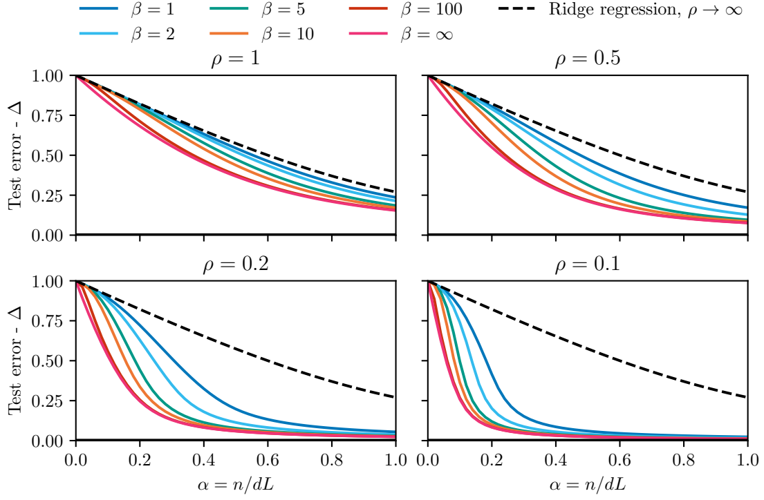
FIG. 8. Same as Figure 2, only with \Delta = 0.1 .
