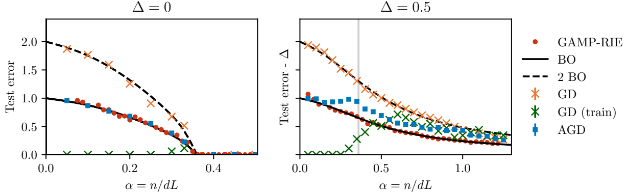
FIG. 5. Comparison between the test error achieved by GD and AGD initialised in the prior and of the BO test error for \beta = 1 , \rho = 0.2 and \Delta = 0, 0.5 (left and right panels respectively). In the noisy case, we depict the test error minus the variance of the noise \Delta . Solid lines are the BO test error, dashed lines are twice the BO test error corresponding to the error of the Gibbs sampler. Orange crosses are numerical experiments for the test errors at the end of the run of GD for d = L = 100 , maximum number of steps \tau = 50000 , and runs are averaged over 16 instances of the data. Blue squares are numerical experiments for the test errors at the end of the run of AGD (averaged over 32 initial conditions) and they are averaged over 2 instances of the data (8 in the right panel up to \alpha = 0.6 ). The error bars denoting standard error on the mean are negligible. In both cases, a fine-tuned value of the learning rate \eta(\alpha) must be used, dependent on the sample ratio \alpha . We provide the values used to generate this plot in Appendix A. The green crosses mark the value of the training loss at the end of the training for GD. The grey vertical line in the right-hand panel marks where the number of samples equals the number of degrees of freedom. Finally, red dots are numerical experiments for GAMP-RIE, with a single random instance of d = L = 100 . We observe that in the noiseless case \Delta = 0 (left), GD achieves a test error compatible with the error of the Gibbs sampler and that AGD achieves a test error compatible with the BO test error. Instead, for \Delta = 0.5 (right) we observe that AGD does not reach the BO error, and moreover it trivialises (namely, all differently-initialised runs of GD converge to the same estimator) for \alpha large enough, roughly around \alpha \approx 1 here. We show qualitatively similar comparisons at \beta = 2 in Appendix A. The Bayes-optimal curves are plotted using Result 2 and (24). The performance of GAMP-RIE, GD and AGD are given by (13) applied to the output of the respective algorithm.
