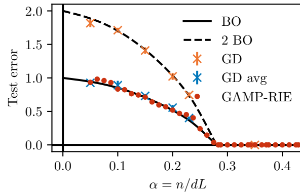
FIG. 10. Same as Figure 5, only with \beta = 2 .
